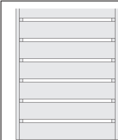
1 x M 1 | 2031 x 606 x 57 mm | ID 93666 2 x M 2 | 2031 x 710 x 57 mm | ID 93665
