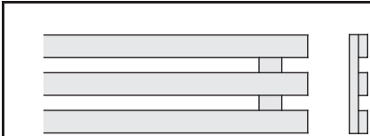
2 x L 3 | 1983 x 174 x 32 mm | ID 38153
