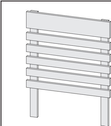
2 x L 4 | 474 x 590 mm | ID 2252 2 x L 5 | 580 x 590 mm | ID 2253
